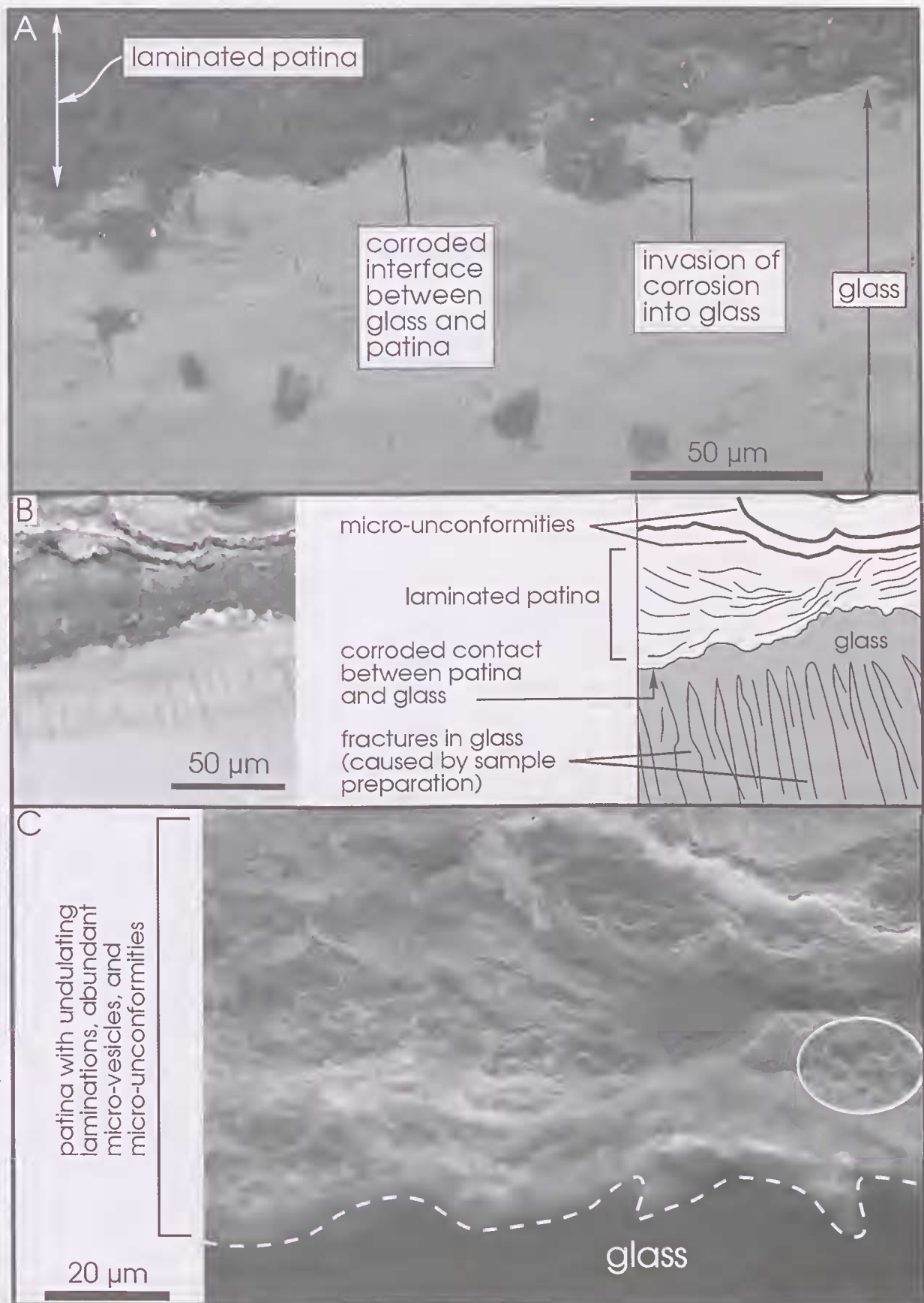
Figure 6. SEM images of a cross-sectional view of patina on glass (sample A2). A. Image shows structureless glass, the corroded interface with the patina, the invasion of corrosion into the glass, and the laminated patina. B. SEM image and annotated line diagram showing corroded contact between glass and patina, undulating lamination in the patina, and micro-unconformities. C. Undulating lamination in the patina, and an abundance of micro-vesicles (one set is circled).
